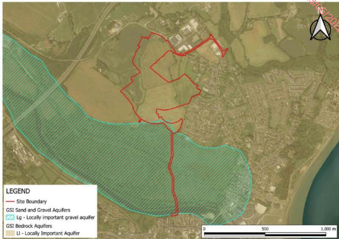
Figure 7.4: Aquifer Classification Map (Source: GSI, 2025)
